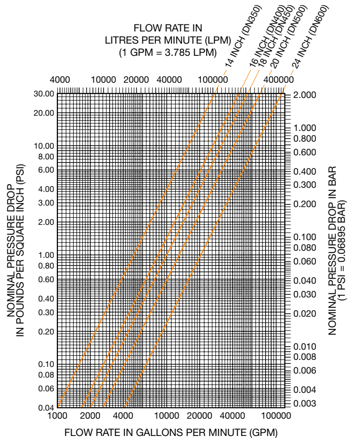
FIGURE CV890 DUAL DISC CHECK VALVE NOMINAL PRESSURE LOSS VS FLOW
