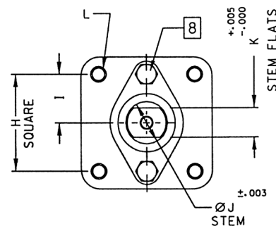
ACTUATOR MOUNTING
